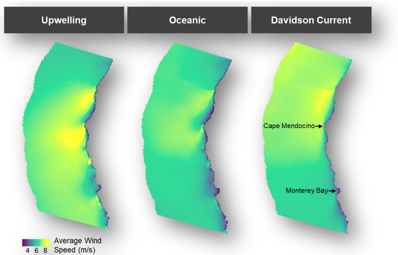
Fig. 10. Offshore windscape for each oceanographic season. The 20-year (2000–2019) wind speed averages (m/s) off California (USA) were derived from CA-20 and Northwest Pacific wind speed models provided by National Renewable Energy Lab. Seasonal averages were calculated based on wind speeds at turbine hub height (150 m above sea level). Data source: National Renewable Energy Lab (2023).
