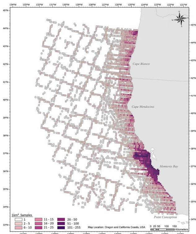
Fig. 5. Distribution of survey effort across the entire study area. Survey effort was quantified by summing the total number of 1 km 2 units of at-sea survey effort, aligned with the resolution of the 2D and 3D prediction grid (5' × 5' cells). The intensity of survey effort at each location is depicted using a color gradient, with darker shades indicating areas of greater survey coverage.
