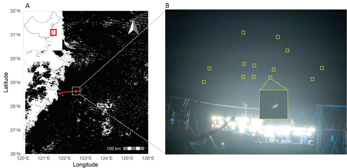
Fig. 1. Observation location and photograph of a light falling-net vessel with a trapped bird flock, operating on 14 October 2025 in the East China Sea (28.63°N, 122.53°E): (A) Trajectory and location of observed vessel (red arrow) with binarized nighttime light base map (data source: Black Marble nighttime lights from NASA, image from the same date; see Román et al., 2018); inset at top left shows the location relative to China (red box). (B) Birds circling inside the light column of the fishing vessel, with individual birds marked by yellow squares. Photo credit: Yu-Xin Lu
